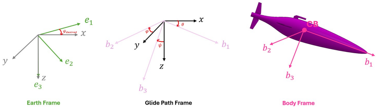
Fig. 4: Coordinate Transformations
